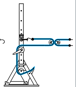
13,60 T Double pull
